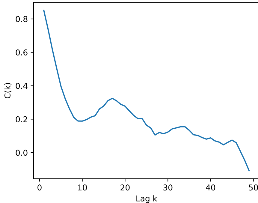
LUMO Autocorrelation
